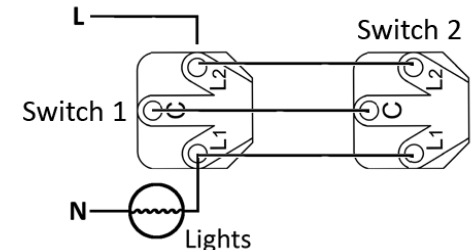
Two-way circuit (type 2)
